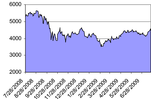
FTSE 100 Index
